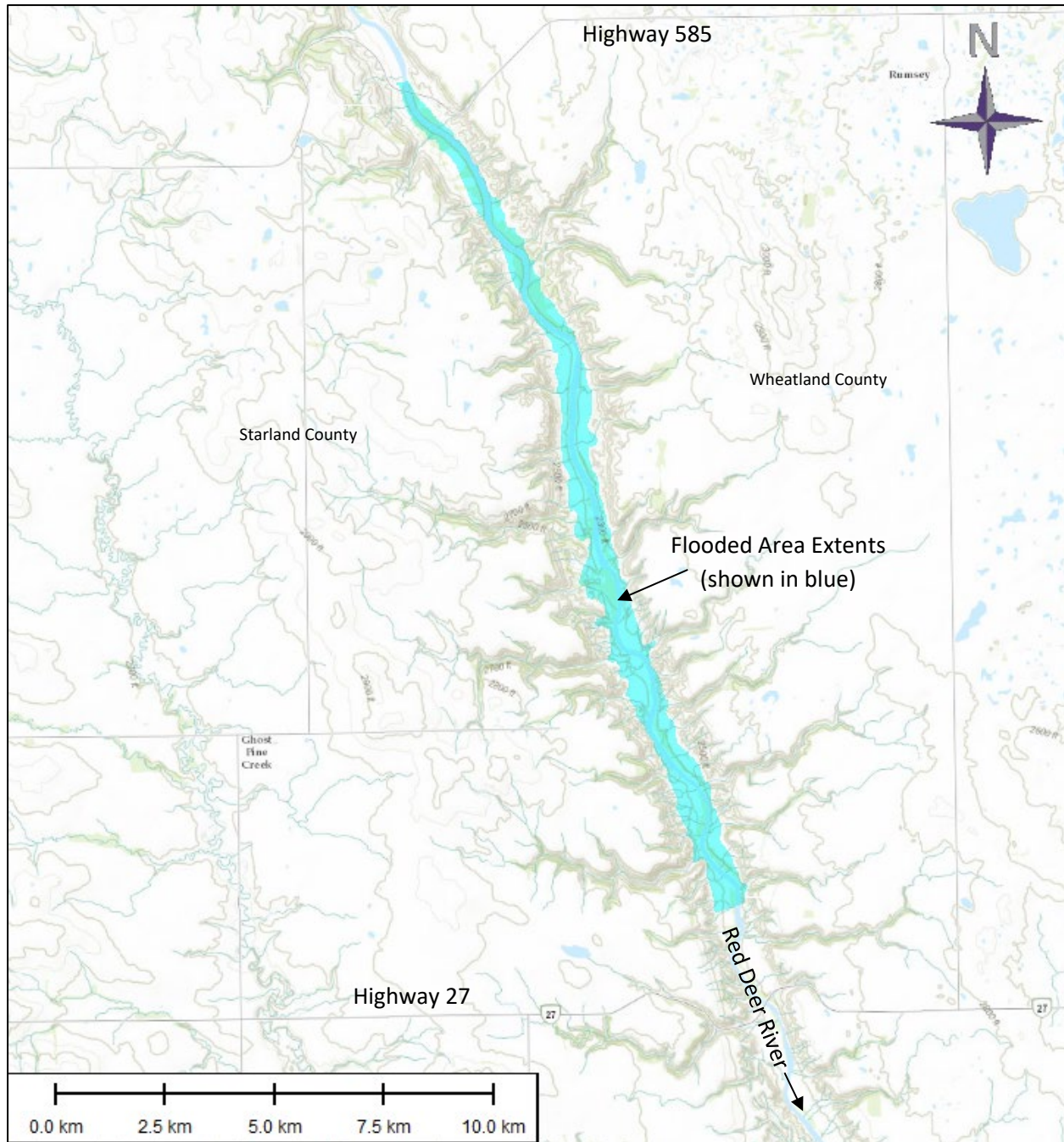
Figure 3: Extent of Flooded Area due to Upstream Storage Reservoir (1:100 flood)
