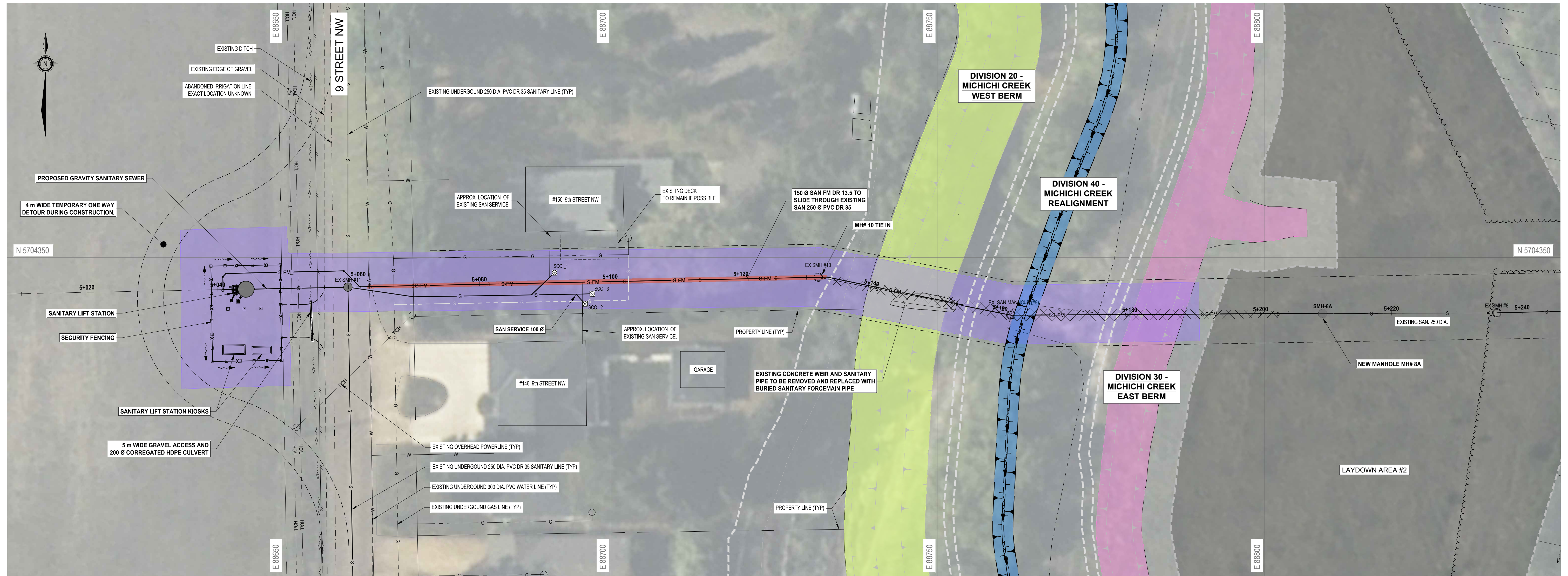
DIVISION 50 - LIFT STATION & FORCEMAIN CROSSING - PLAN
